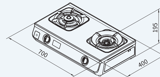
G5920AS
