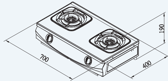
G5900S
