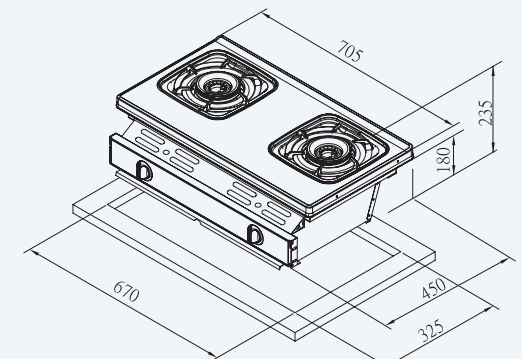
G6900S
