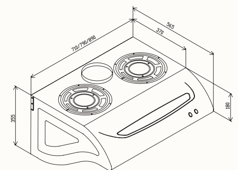
R3250
