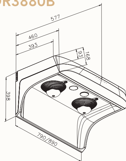
DR3880B
